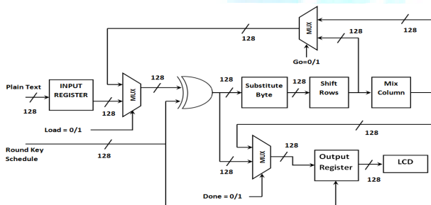
Figure 2.1 AES Encryption Block Diagram
